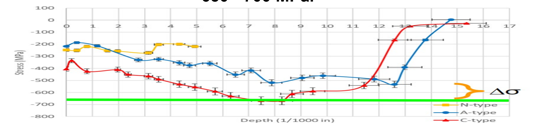
Figure 8: Stress-Depth profiles under Perp. High conditions and how the maximum compressive stresses compare to half of the 1070 steel yield stress of 1300-1400 MPa.
